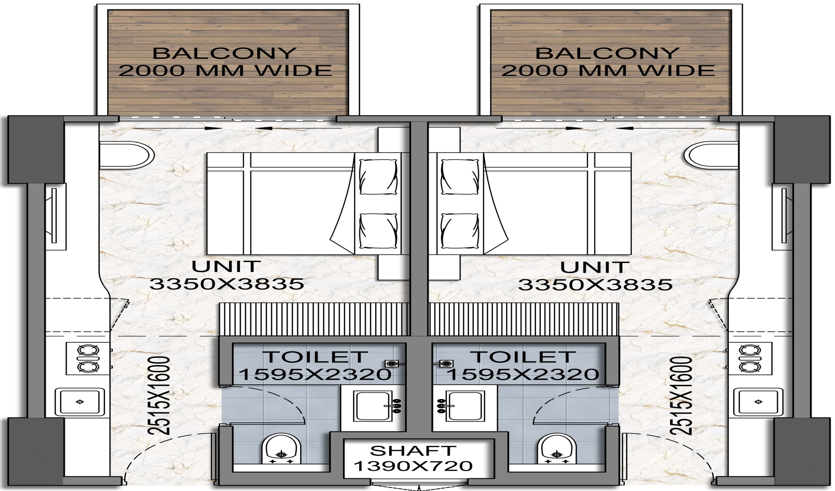
TYPICAL UNIT
